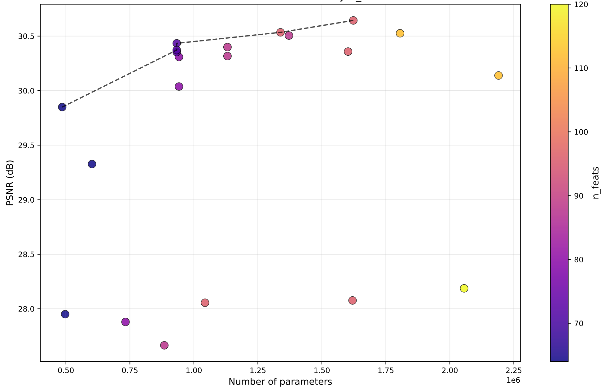
PSNR vs #Params — ELAN — by n_feats
